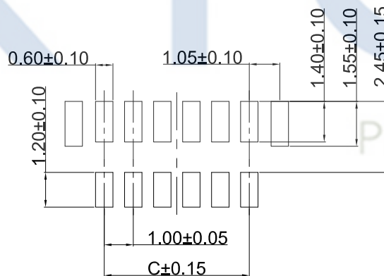
Board Layout
